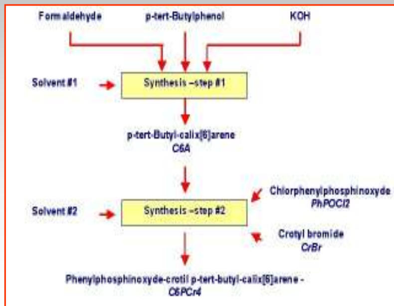
Synthesis route
